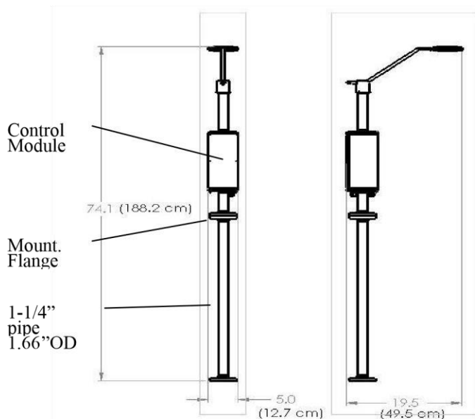
Mechanical Interface: 72"H x 22"W
