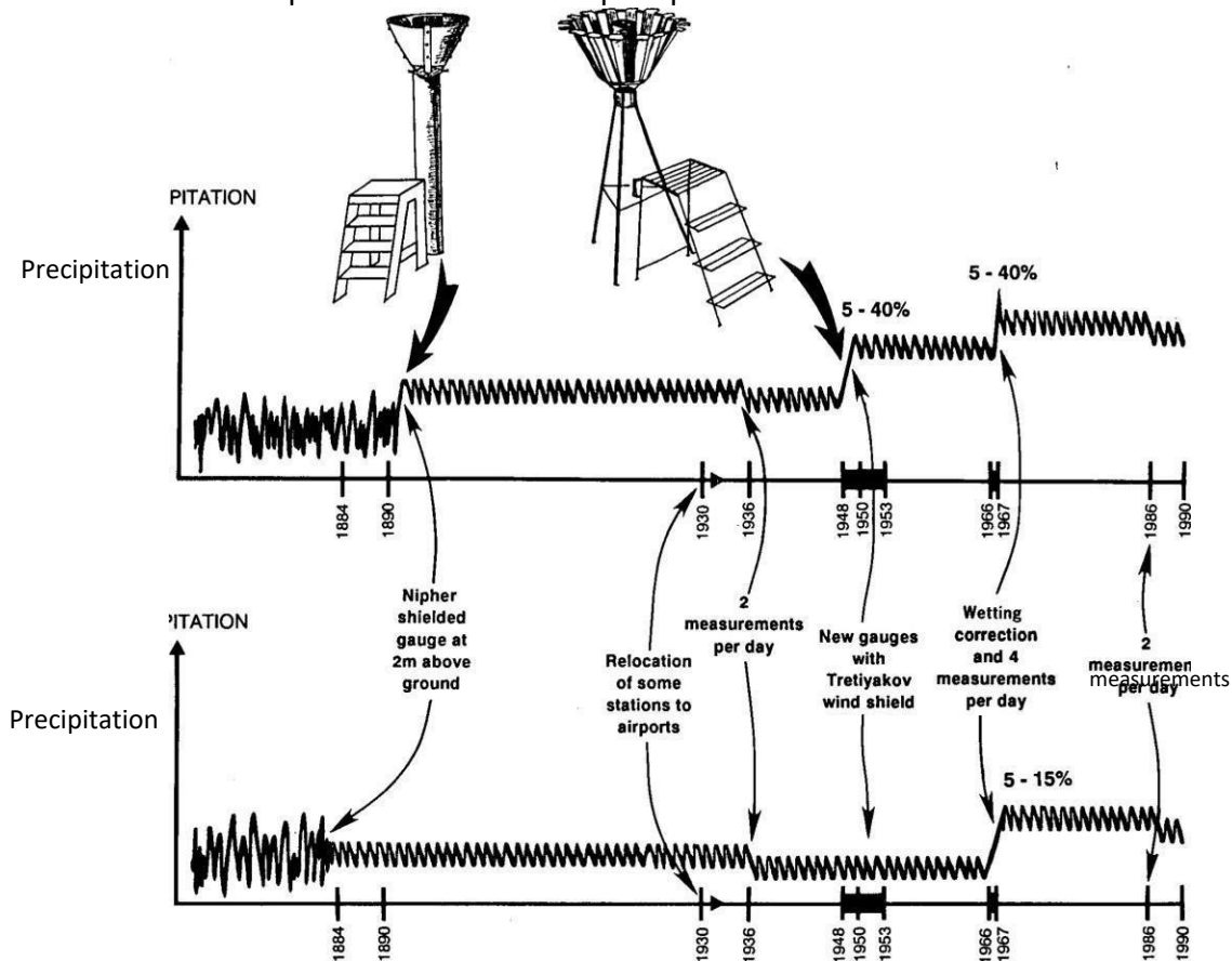
FIG. 1. An illustration depicting the systematic changes in the precipitation network over the USSR (Groisman et al. 1991)
