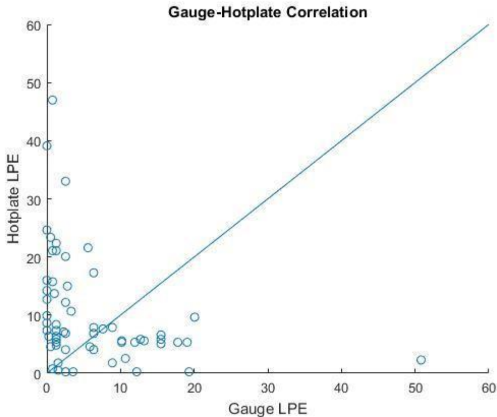
FIG 5: Hotplate and Gauge LPE correlation relative to a 1:1 line
