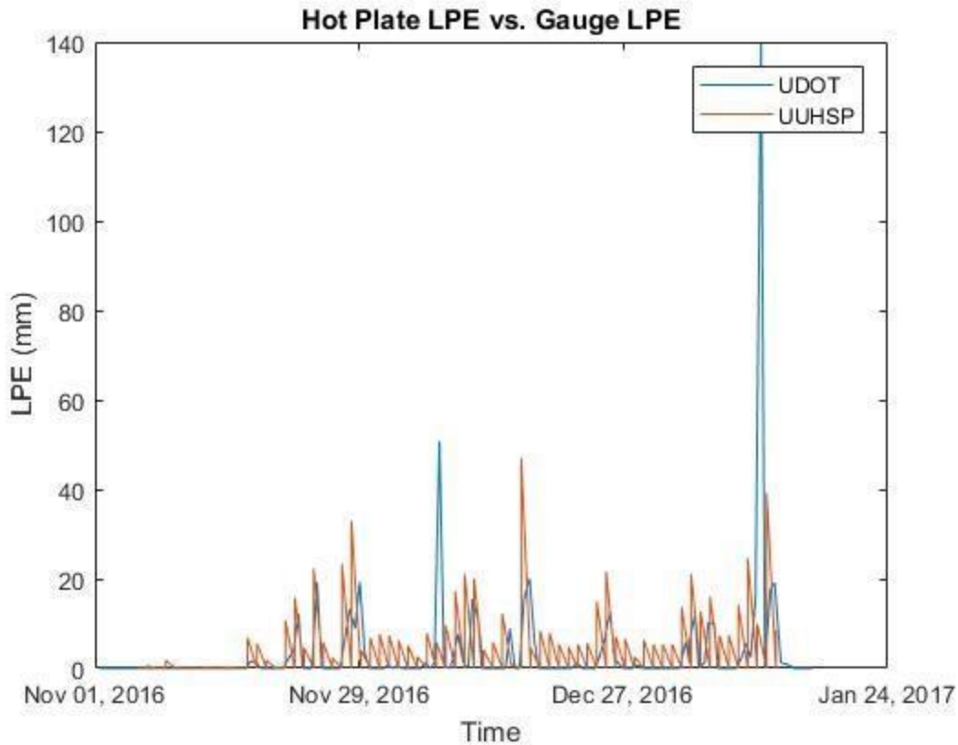
FIG 4: LPE output (mm) of the gauge and hotplate during time hotplate communications were active
